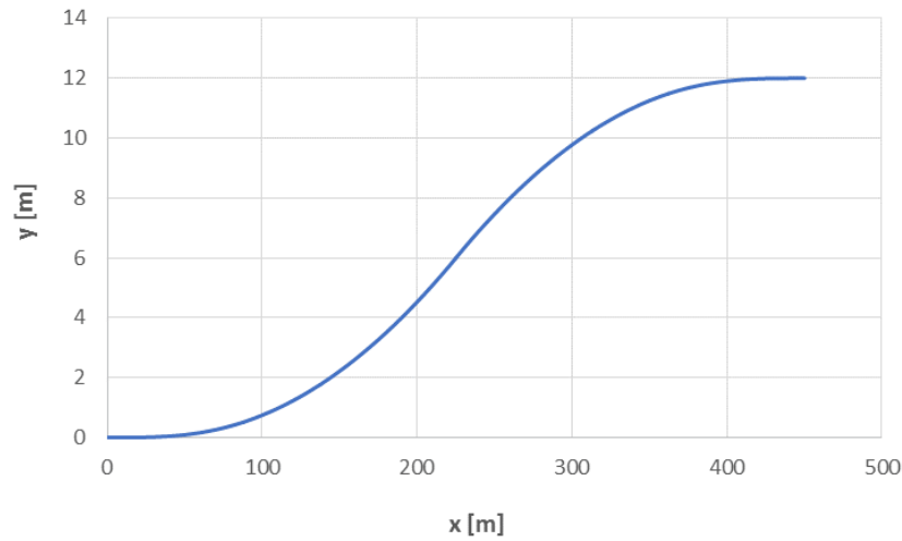
Fig. 9. Diagram of horizontal ordinates along the length of the determined intertrack space widening ( k = 1/3000 \text{ rad/m} , l_1 = l_3 = 88 \text{ m} , l_2 = 49.212 \text{ m} , in non-comparative scale)
