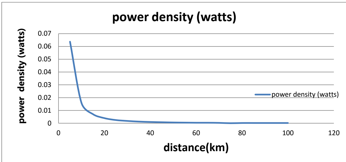
Fig. 3. Effect of transmitter gain on power density
