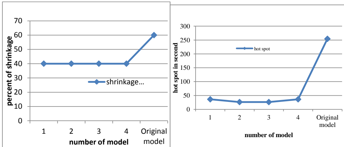
Fig. 10 (a, b) Result of runner optimization for shrinkage porosity and hospot runner
