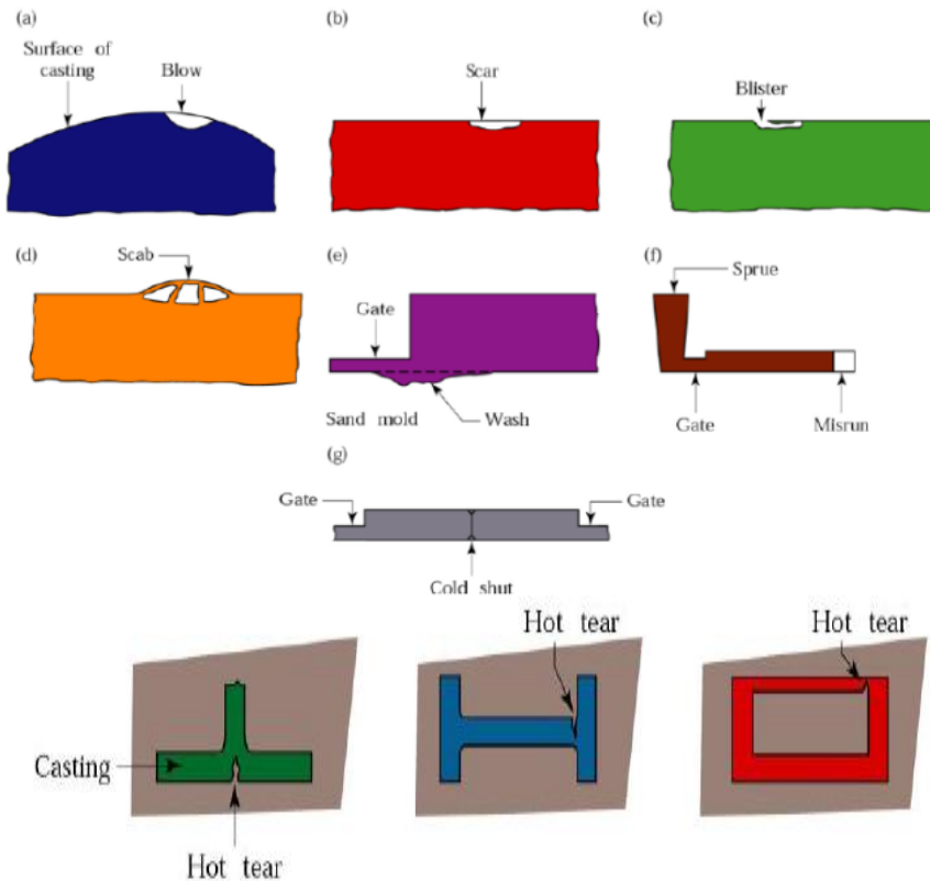
Fig. 3. Defects observed in aluminium and it alloys by using sand casting process
