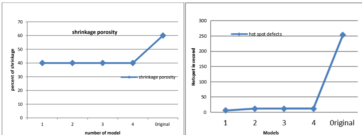
Fig. 14 (a,b). Simulation result of ingate optimization parameter with shrinkage porosity
