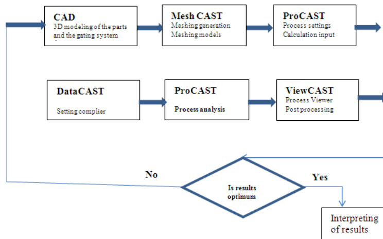
Fig. 7. Flow chart of simulation work on Pro-CAST
