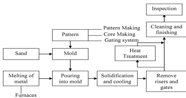
Fig. 1. Production steps in a typical sand casting process.
