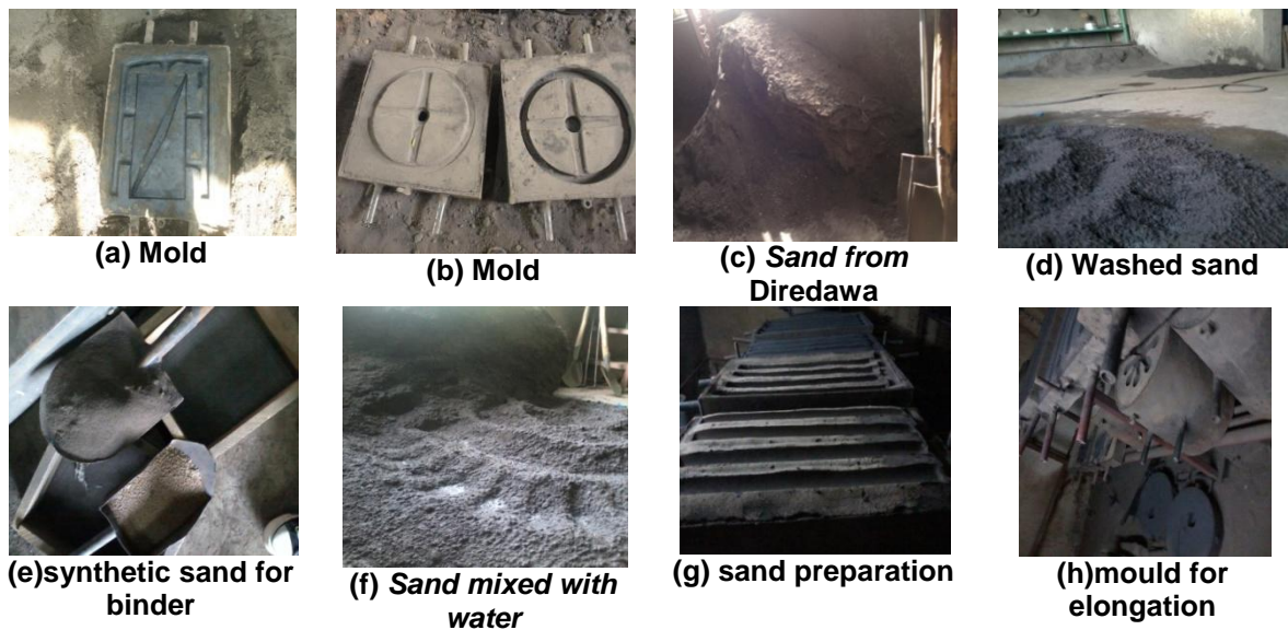
Fig. 4. (a-h) Mold and sand preparation methods for molten metals pouring
