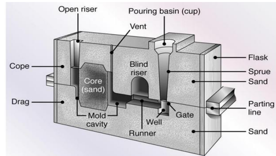
Fig. 2. Element of gating system in sand casting process
