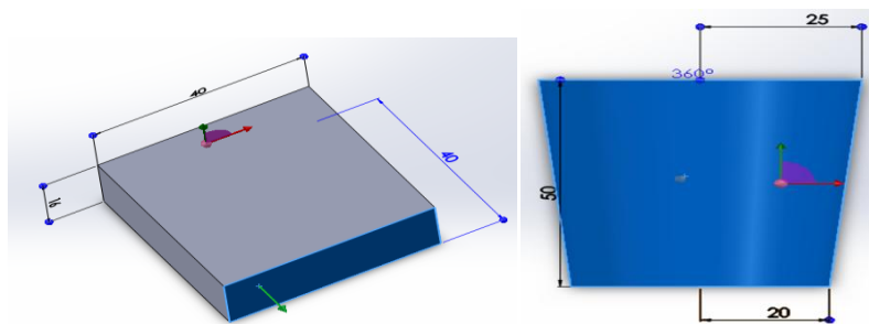
Fig. 9. (a,b) Optimization of Ingate and Riser
