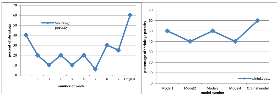
Fig.12 (a,b). Results of Shrinkage Porosity on number of models and first phase optimization
