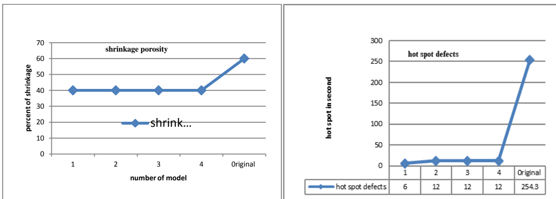
Fig. 11 (a,b). Simulation result of Ingate optimization parameter with shrinkage porosity
