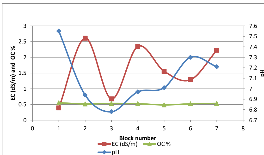
Fig. 2. Physico-chemical parameters of different soil in TNU
