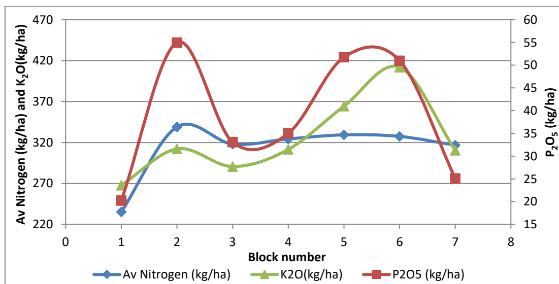
Fig. 3. Macro nutrient content of different soil in TNU
