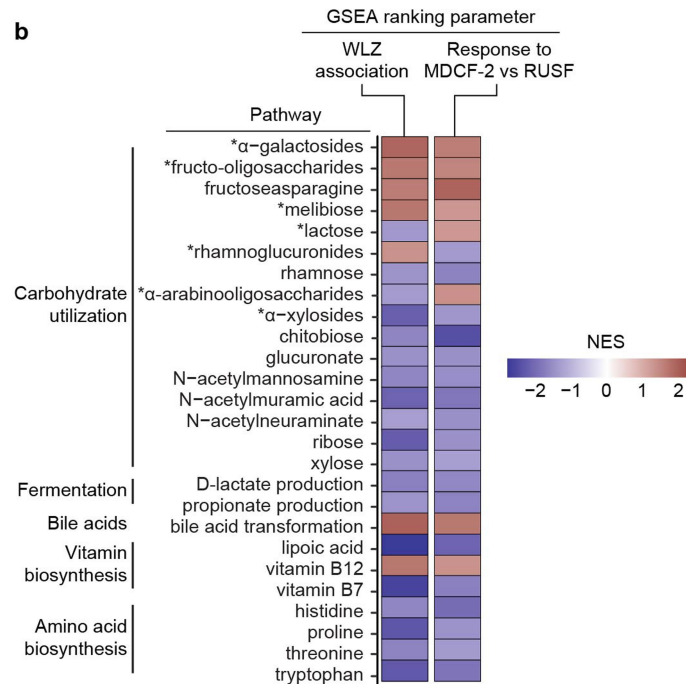
Extended Data Fig. 2 | Taxonomy and functional characteristics of WLZ-associated MAGs. (a) Left subpanel, density plot showing WLZ-associated MAGs tabulated based on their genus-level classification. \beta_1 refers to the coefficient in the linear mixed effects model presented at the bottom of the figure. Genera containing >3 significantly WLZ-associated MAGs are shown. Right subpanel, number of statistically significant WLZ-associated MAGs assigned to each genus depicted in the left subpanel. (b) Enrichment of metabolic pathways in WLZ- and treatment-associated MAGs. MAGs were
