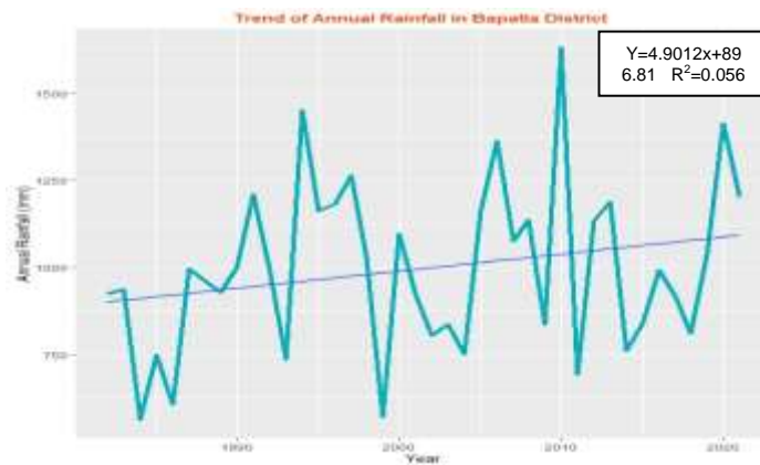
Fig. 3. Trend of annual rainfall of Bapatla district from 1982 to 2021
