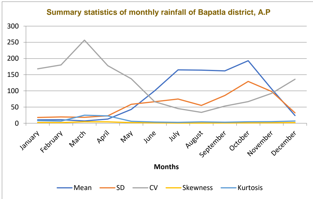
Fig. 1. Descriptive statistics of monthly rainfall pattern of Bapatla district, A.P
