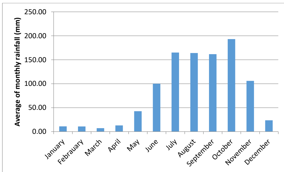
Fig. 2. Average monthly rainfall of Bapatla district, A.P
