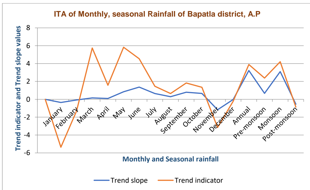
Fig. 4. Trend indicator and Trend slope of Innovative trend Analysis
