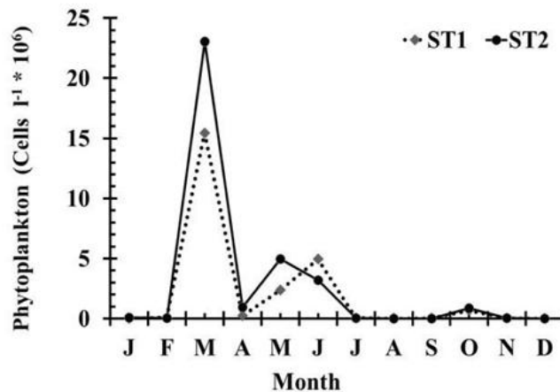
Fig. 8. Variations of phytoplankton abundance during research period
