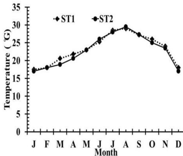
Fig. 2. Variations of temperature during research period
