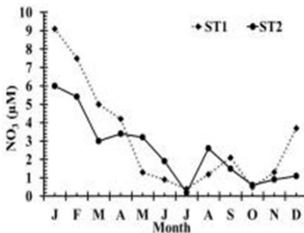
Fig. 4. Variations of nitrate during research period
