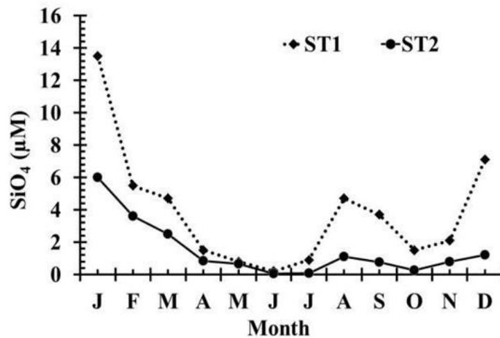
Fig. 5. Variations of silicate during research period
