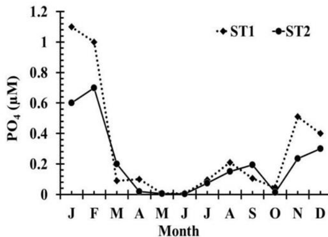
Fig. 6. Variations of phosphate during research period
