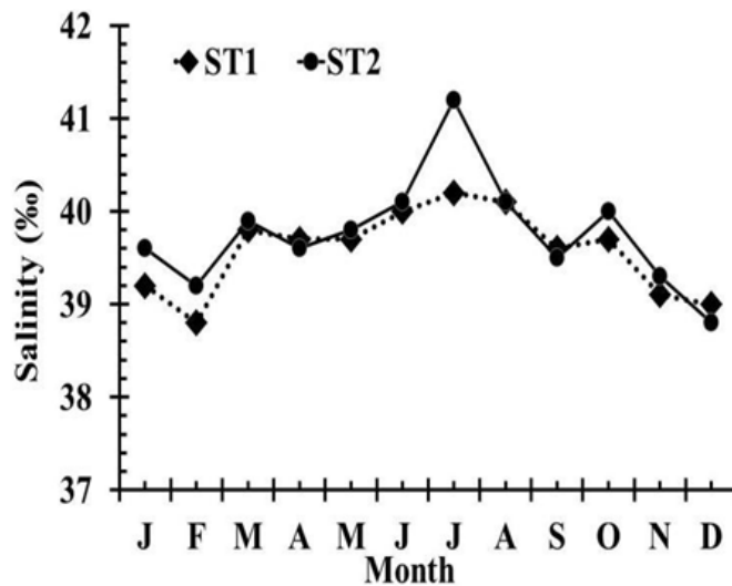
Fig. 3. Variations of salinity during research period
