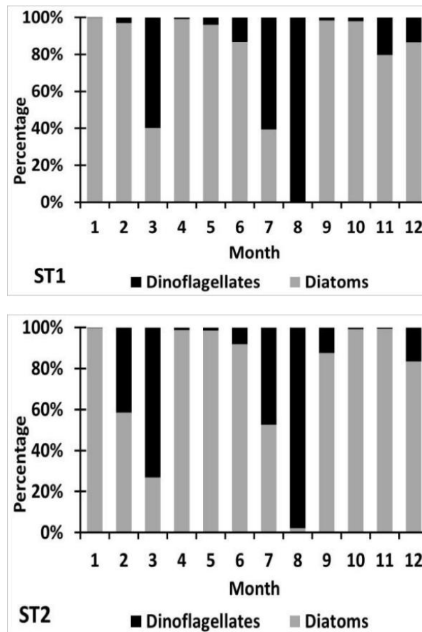
Fig. 9. Presence of dinoflagellates and diatoms in 2 sites
