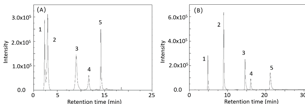
Fig. 1. The chromatogram of five standards with empirical LC method (A) and optimized LC method (B)
