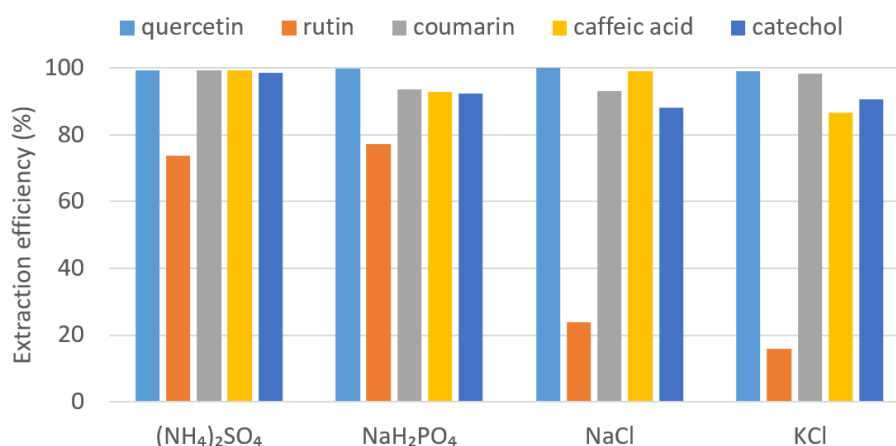
Fig. 2. Extraction efficiency with different salts
