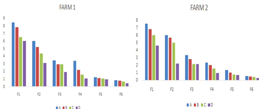
Fig. 6. Concentration of Zinc. A = 3 mm-deep dry sediment [flooded area]; B = 30 cm deep; not including dry sediment [flooded area] C = 3 mm-deep surface soil [non-flooded area]; D = 30 cm deep; not including surface soil [non-flooded area]. Y-axis = concentration of metal in mg/kg
