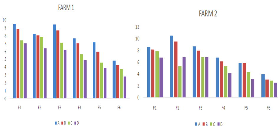
Fig. 7. Concentration of iron. A = 3 mm-deep dry sediment [flooded area]; B = 30 cm deep; not including dry sediment [flooded area] C = 3 mm-deep surface soil [non-flooded area]; D = 30 cm deep; not including surface soil [non-flooded area]. Y-axis = concentration of metal in mg/kg
